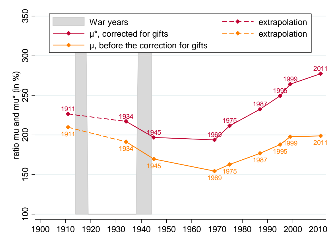
Figure 1: Evolution of \mu_t and \mu_t^*
