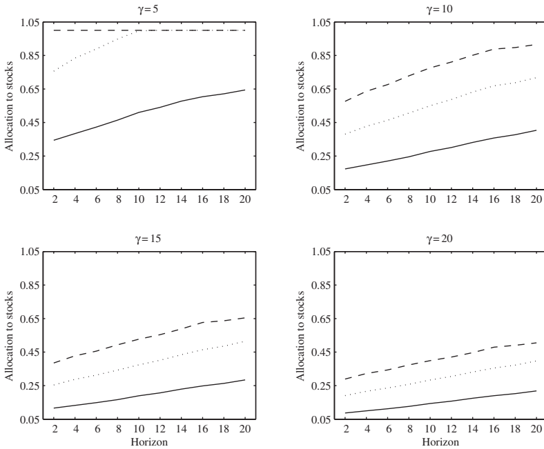
Figure 1 Horizon effect
