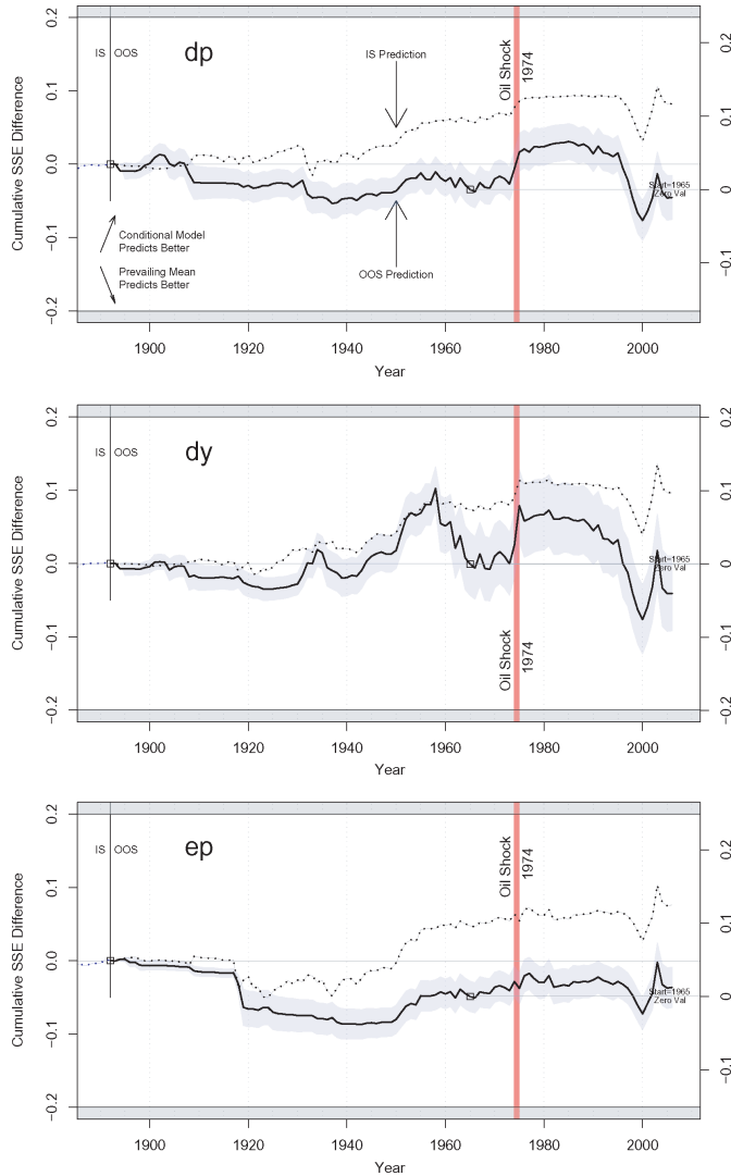
Figure 1 Annual performance of IS insignificant predictors. Explanation: These figures plot the IS and OOS performance of annual predictive regressions. Specifically, these are the cumulative squared prediction errors of the NULL minus the cumulative squared prediction error of the ALTERNATIVE. The ALTERNATIVE is a model that relies on predictive variables noted in each graph. The NULL is the prevailing equity premium mean for the OOS graph, and the full-period equity premium mean for the IS graph. The IS prediction relative performance is dotted (and usually above), the OOS prediction relative performance is solid. An increase in a line indicates better performance of the named model; a decrease in a line indicates better performance of the NULL. The blue band is the equivalent of 95% two-sided levels, based on MSE-T critical values from McCracken (2004). (MSE-T is the Diebold and Mariano (1995) t -statistic modified by Harvey, Leybourne, and Newbold (1998)). The right axis shifts the zero point to 1965. The Oil Shock is marked by a red vertical line.
